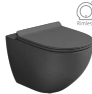
S122021156 KATY BL Product : Wall Hung Closet Dimension : 540x365x360mm Flush System : Rimless Washdown Blind Installation with fittings kit Seat Cover : UF Soft Close Colour/Finish : Black Satin Matt MRP : ₹21990
